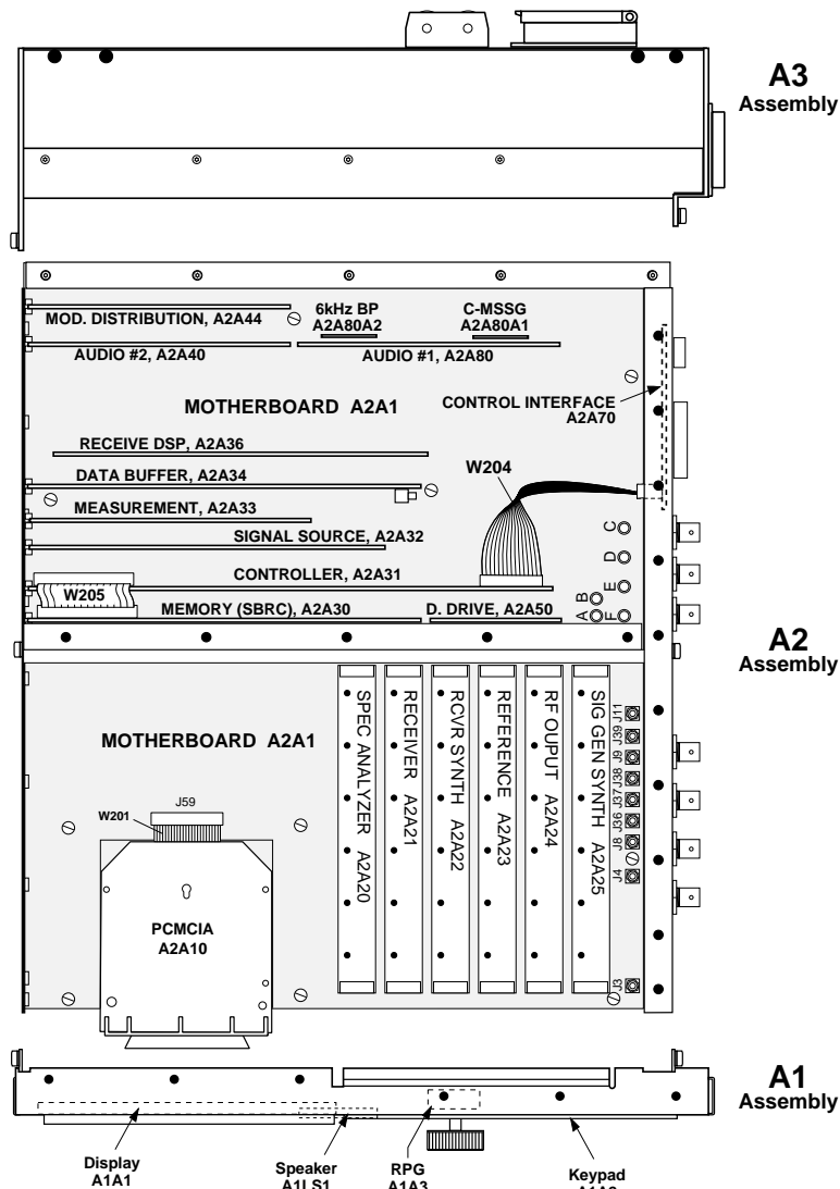
Figure 6-1 Major Assemblies
